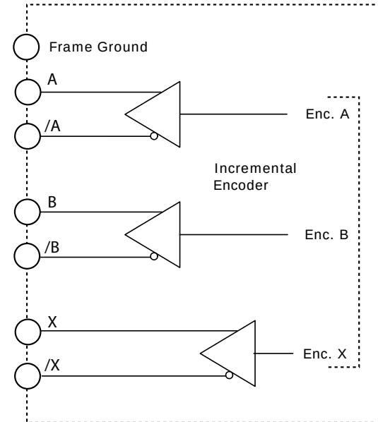
J1 Multi-Port
