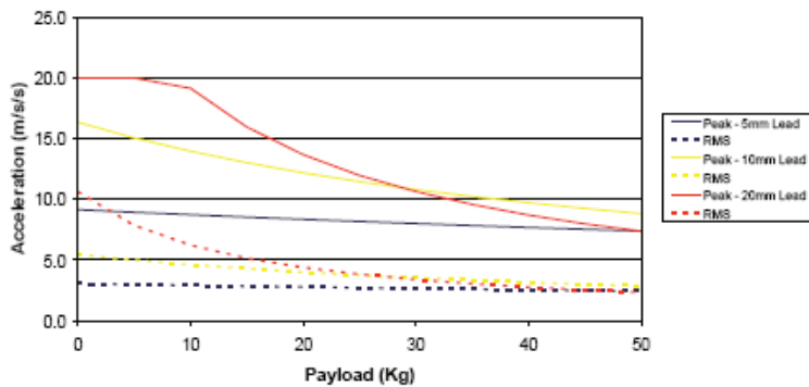
Motor Characteristics
