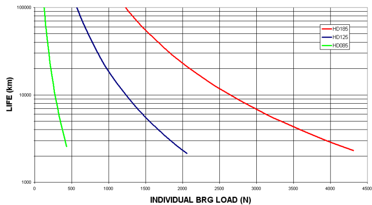
HD SERIES BRG LIFE VS. LOAD (SIDE)
