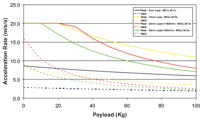
Motor Characteristics
