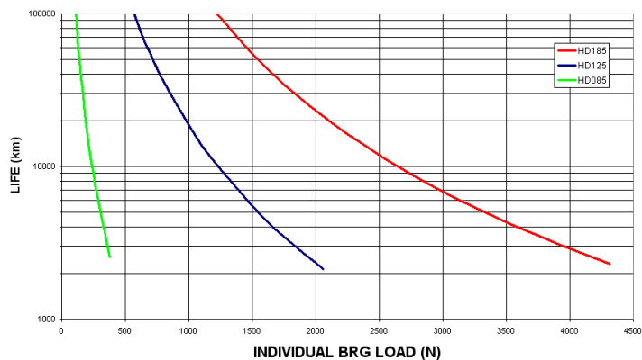
HD SERIES BRG LIFE VS. LOAD (SIDE)
