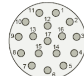
Feedback Connector # 43-025367-01 (Mating Conn.# 43-021660-01)
