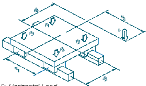
Figure 2: Horizontal Load
