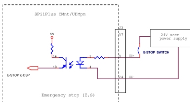
Figure 1-16. Emergency stop input
