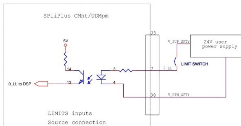
Figure 1-15. Limit connections
