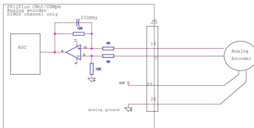
Figure 1-23. Sin-Cos encoder connections
