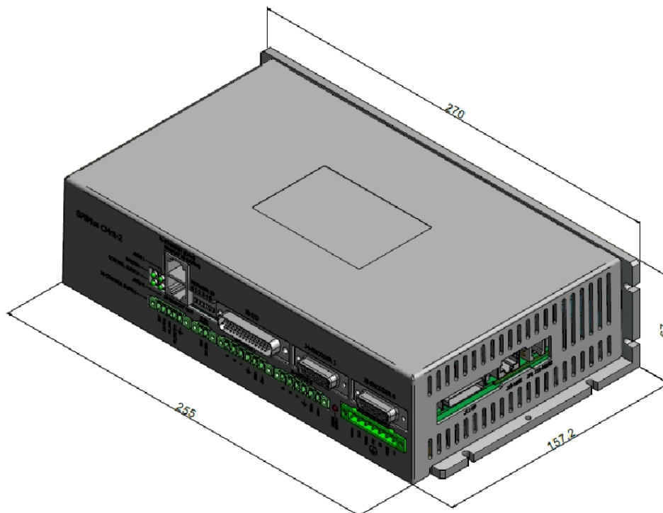
Figure 1-35. SPIIPlusCMnt dimensions
