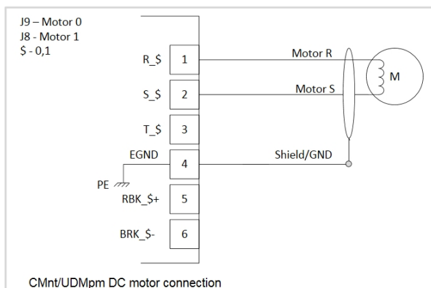
Figure 1-29. DC brush motor connection
