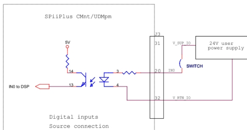
Figure 1-17. Digital input connections
