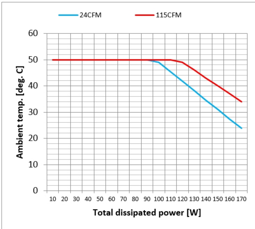
Figure 1-39. Dissipated power vs temperature
