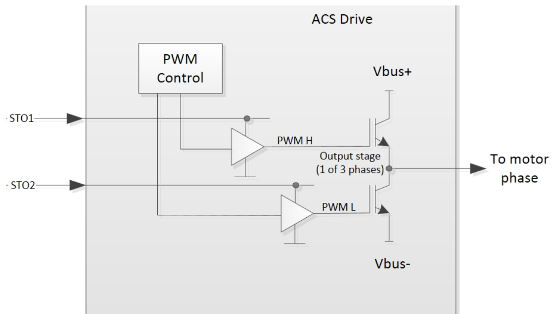
Figure 1-20. STO implementation
