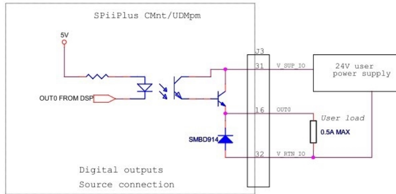
Figure 1-18. Digital output connections
