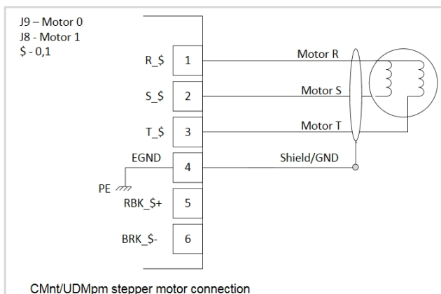
Figure 1-30. Two-phase motor connection
