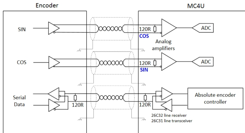
Figure 1-25. Absolute encoder schematic diagram
