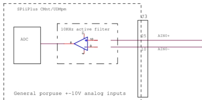
Figure 1-14. General purpose analog inputs
