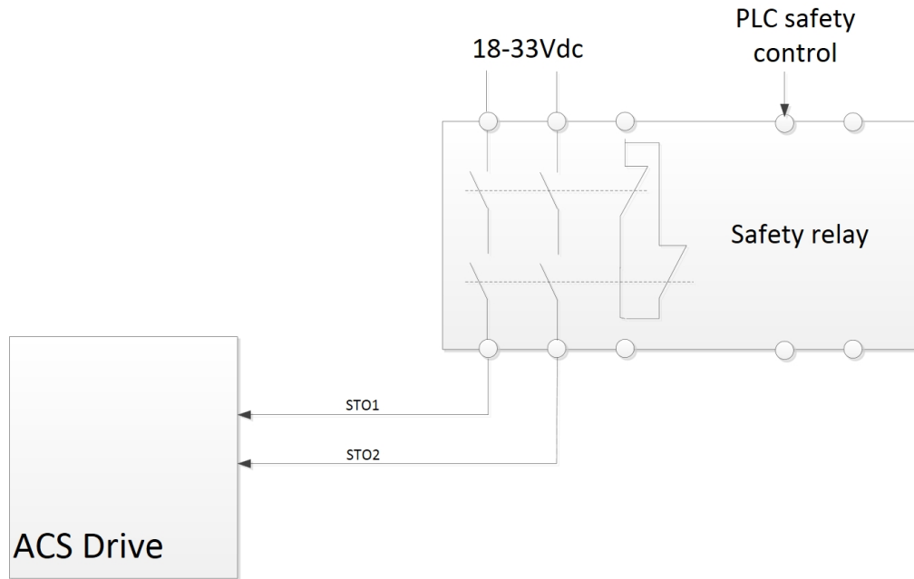
Figure 1-19. STO wiring scheme
