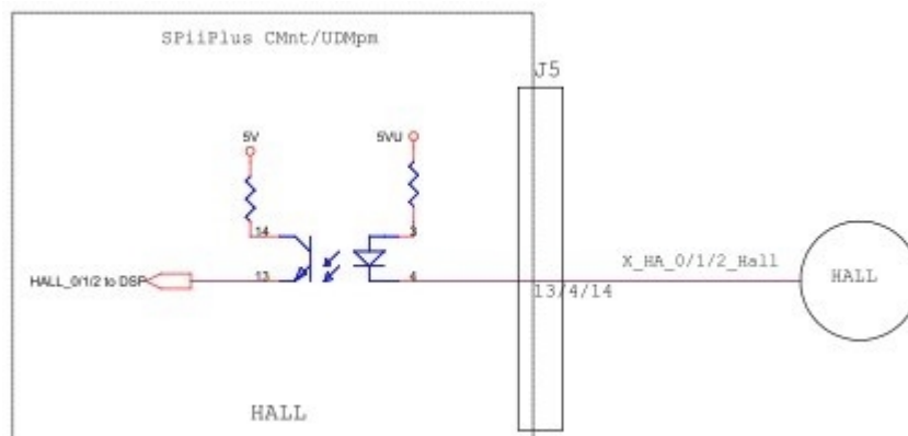
Figure 1-22. Hall sensors connection
