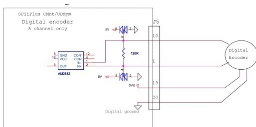
Figure 1-21. Incremental digital AqB encoder connections
