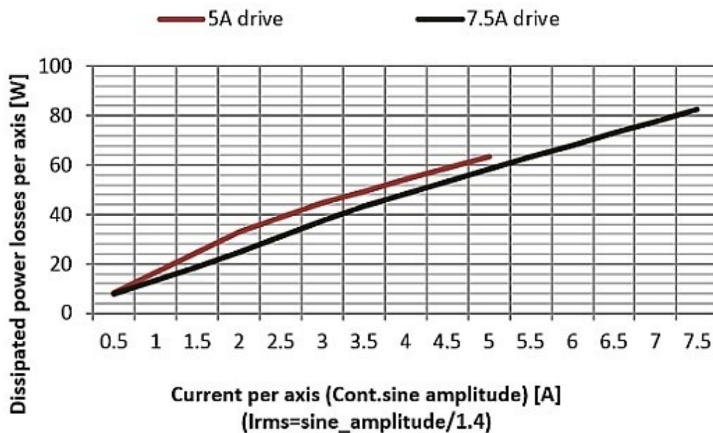
Figure 1-37. Dissipated power vs current
