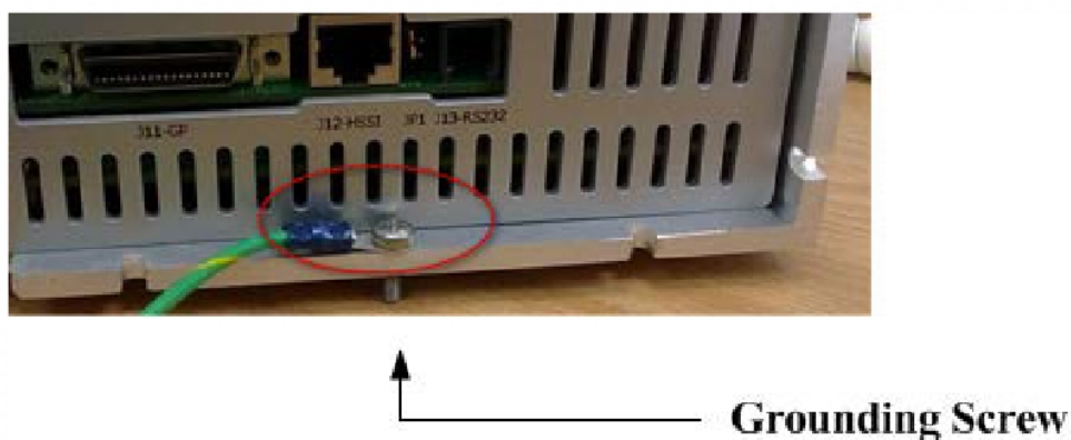
Figure 1-11. Grounding screw
