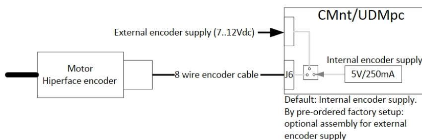
Figure 1-27. External power connection
