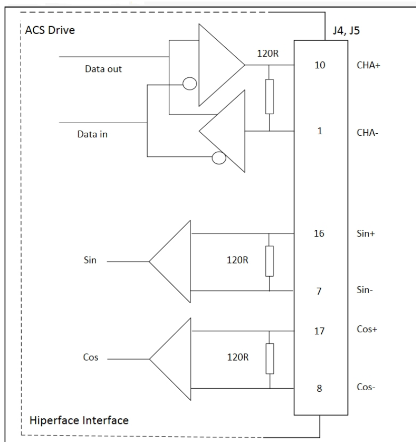
Figure 1-24. Absolute encoder hiperface schematic diagram
