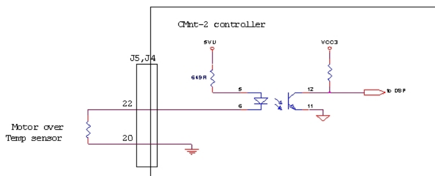
Figure 1-31. Motor over temperature connection
