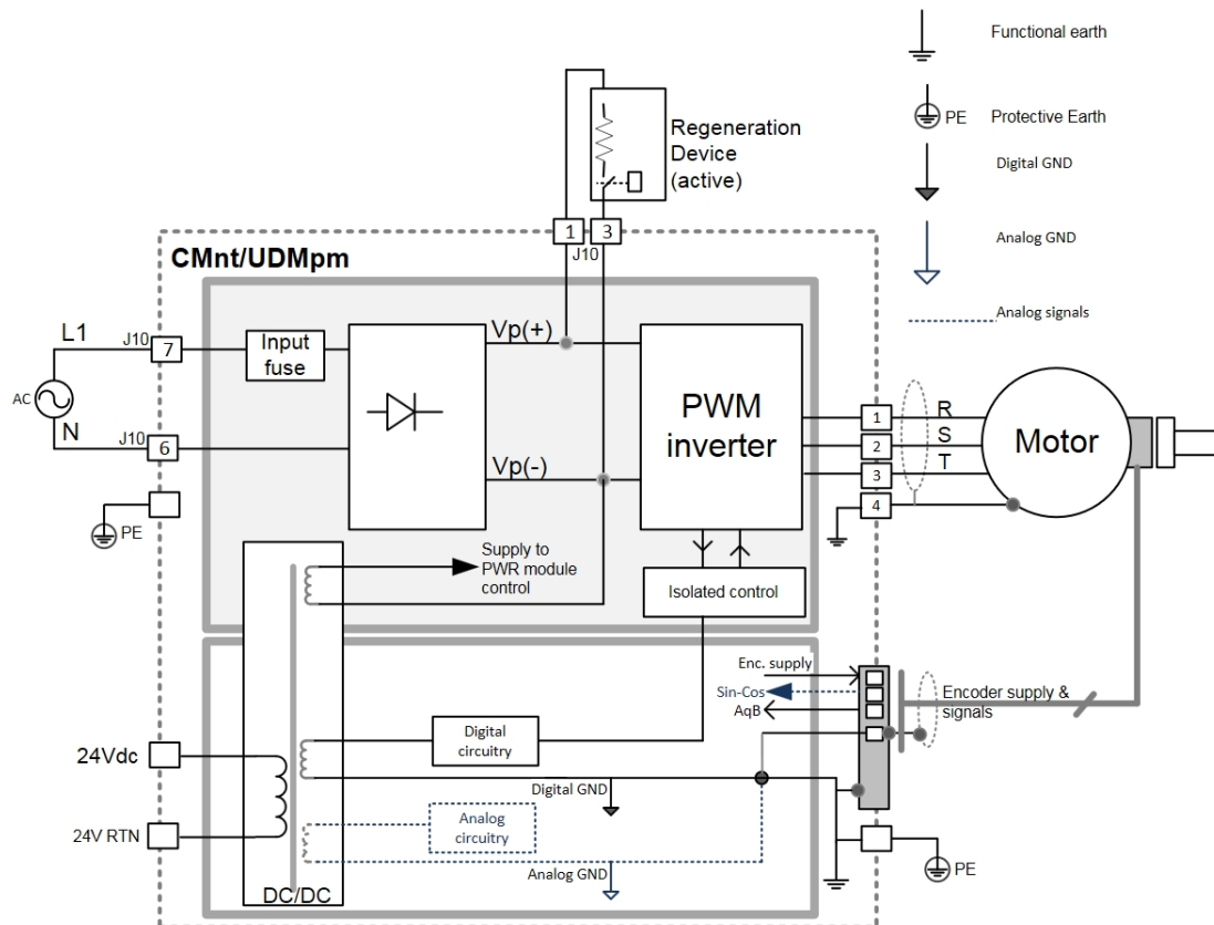
Figure 1-12. Grounding and shielding
