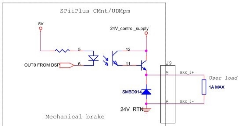
Figure 1-33. Mechanical brake
