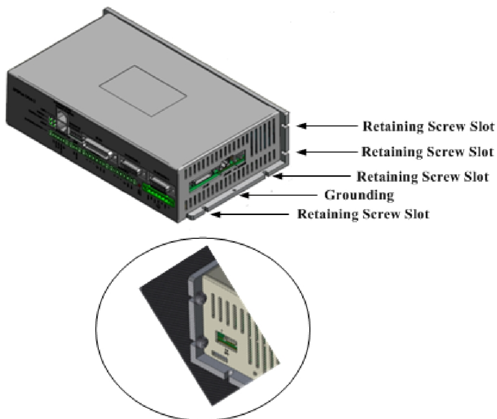
Figure 1-10. Retaining screw locations
