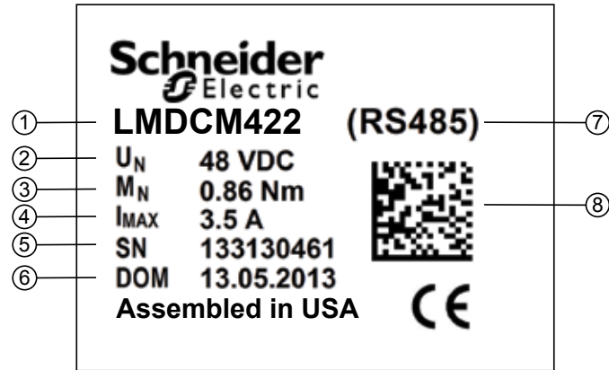
Figure 1.2: Name plate
