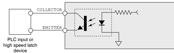
Figure 6.9: Signal output
