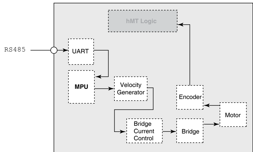
Figure 8.5: Motion block, hMT disabled
