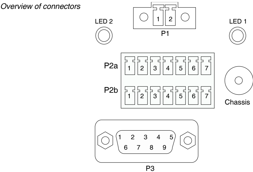
Figure 6.1: Overview of connectors
