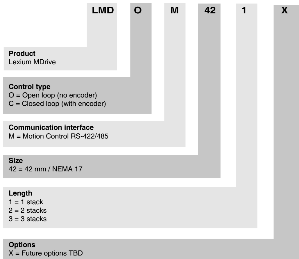
Figure 1.3: Part numbering
