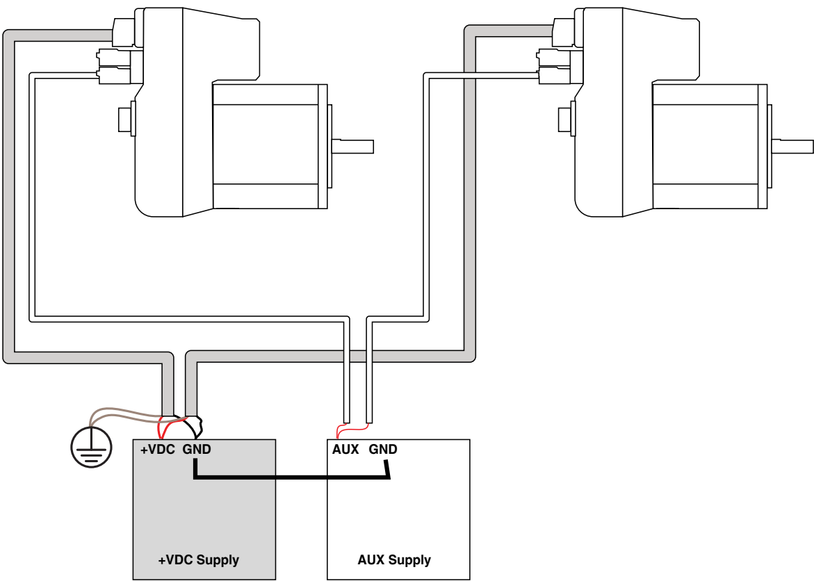
Figure 5.4: System power wiring
