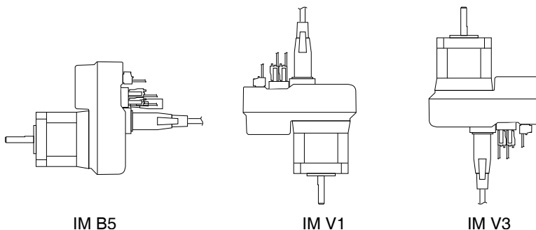
Figure 3.1: Mounting positions
