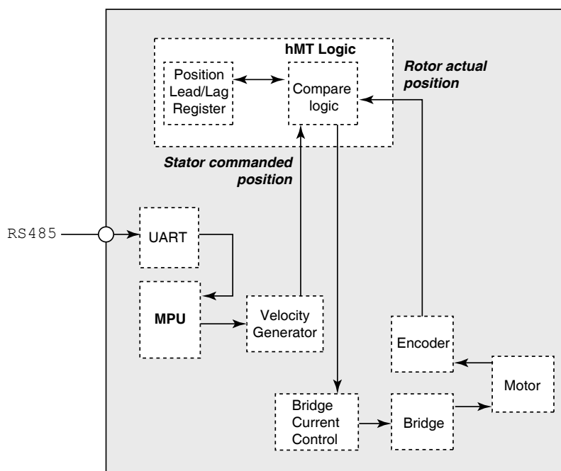
Figure 8.6: Block diagram, hMT enable (AS=1/2)
