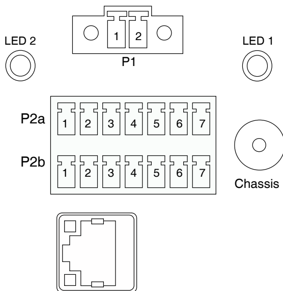
Figure 3.4: Overview of connectors
