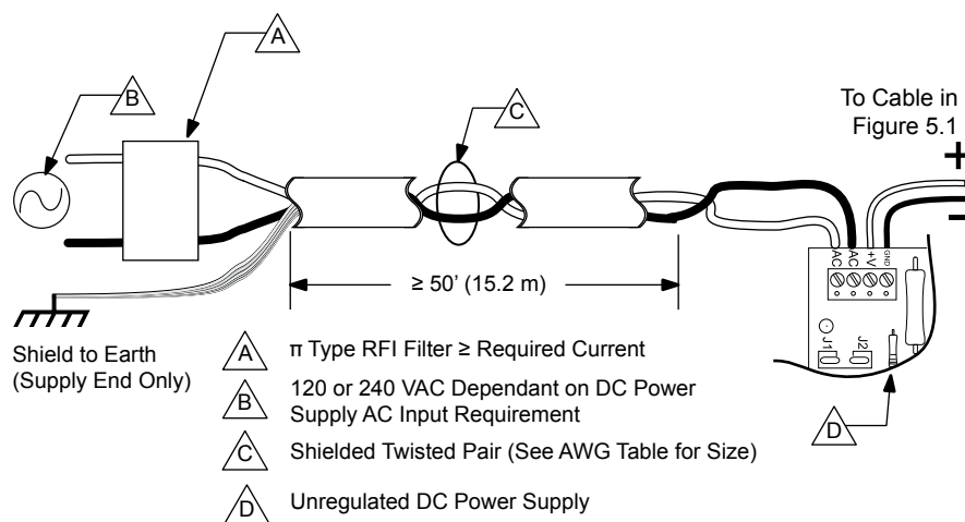
Figure 5.3 50' (15.2 m) or greater, AC power to DC supply
