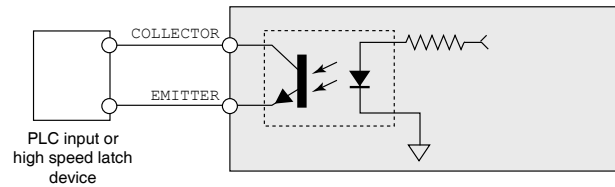
Figure 6.9: Signal output
