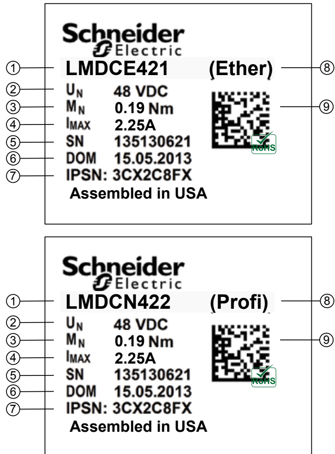
Figure 1.2: Name plate
