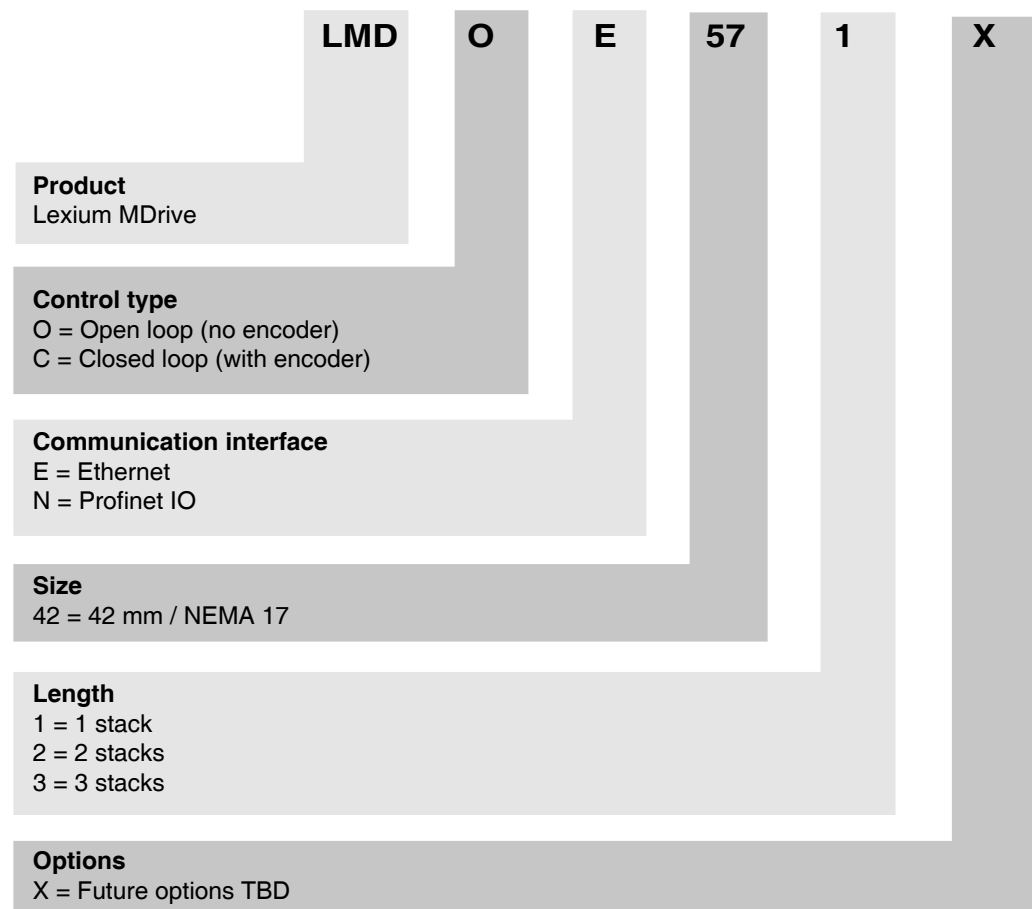
Figure 1.3: Part numbering
