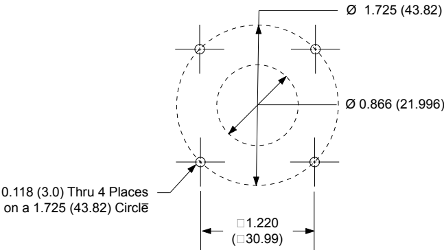
Figure 3.2: Mounting hole pattern (not to scale)
