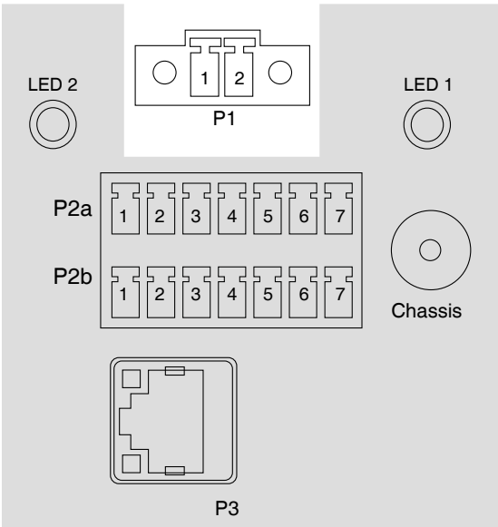
Figure 6.2: Pin Assignment supply voltage
