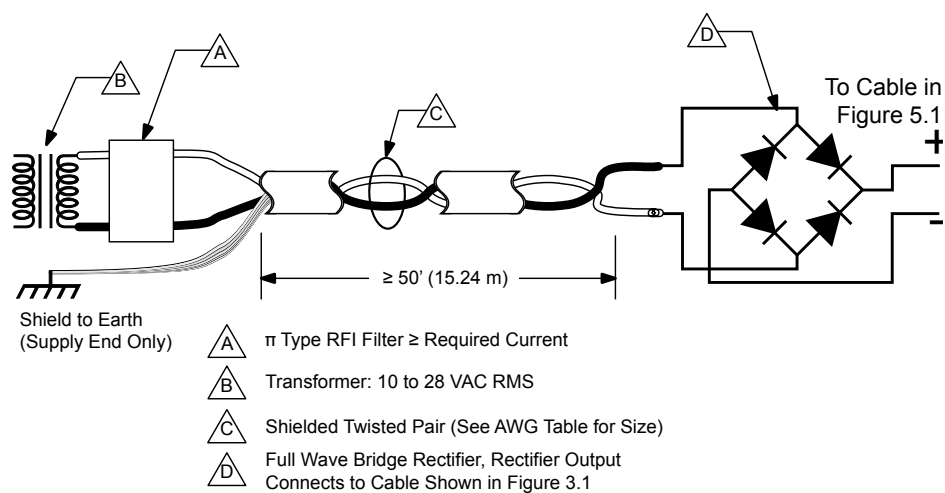
Figure 5.2 50' (15.2 m) or greater, AC power to full wave bridge
