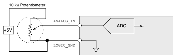
Figure 6.10: ANALOG_IN signal input
