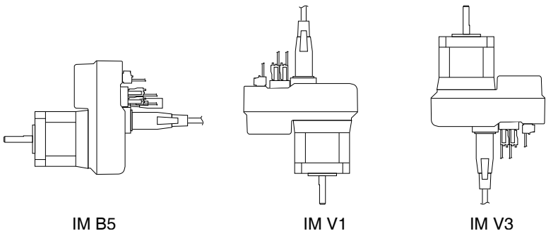
Figure 3.1: Mounting positions
