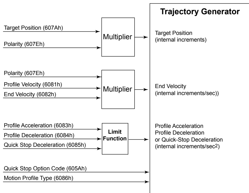
Figure 6.2: Trajectory generator for profile position block diagram
